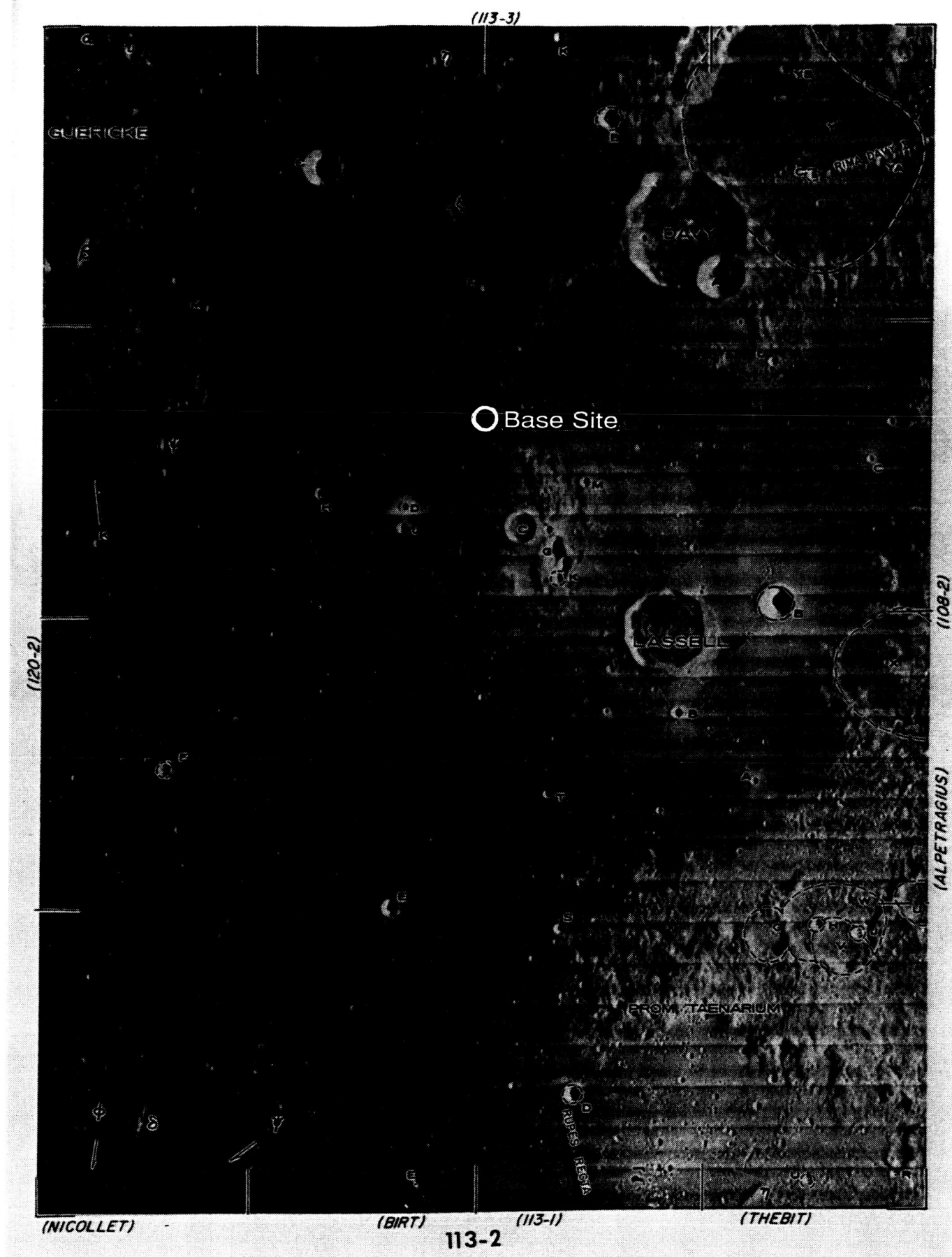
Figure 2.2-2, Mare Nubium Landing Area
