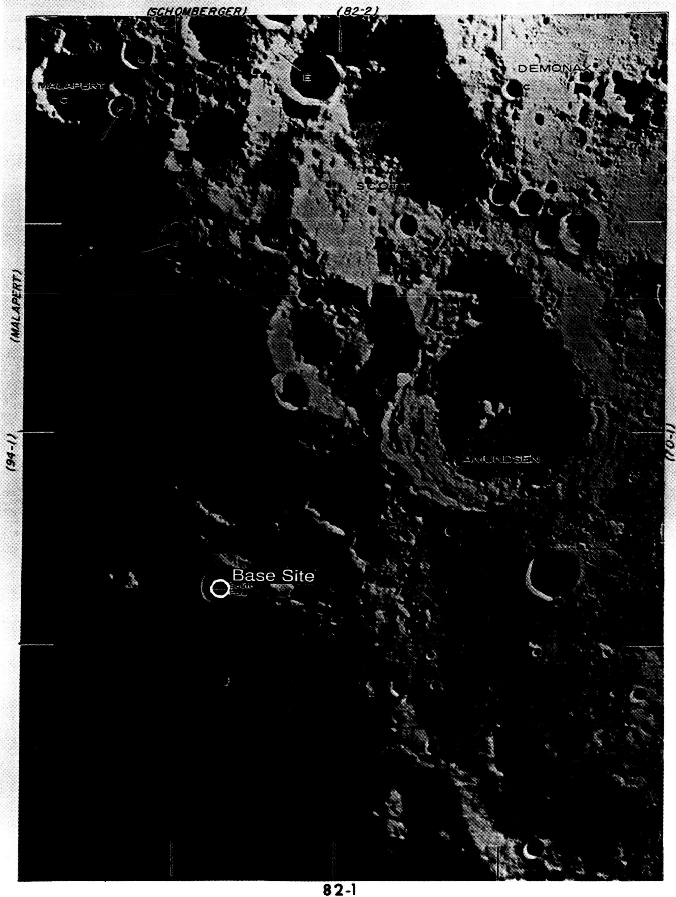
Figure 2.2-6, South Pole Landing Area
