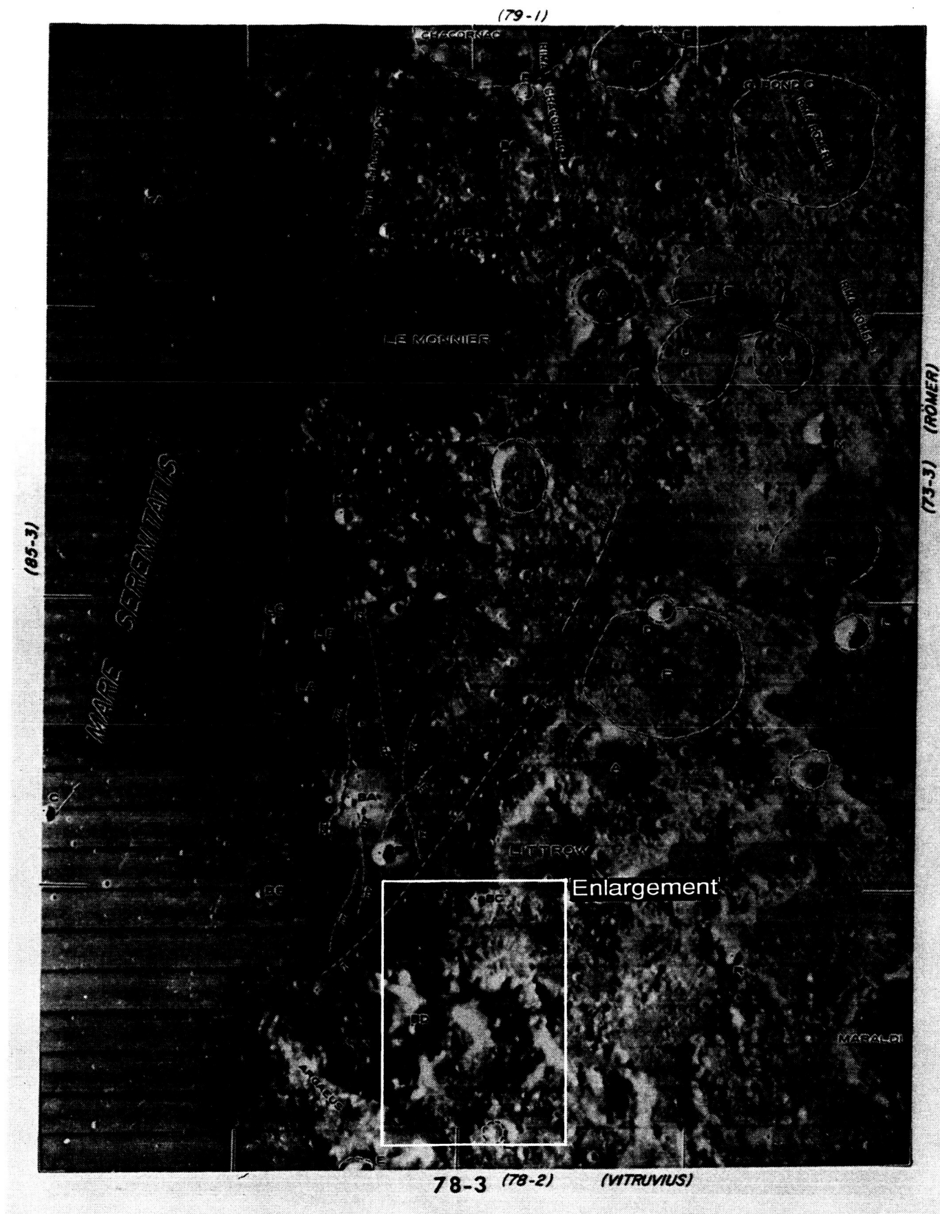
Figure 2.2-3, Taurus-Littrow Landing Area
