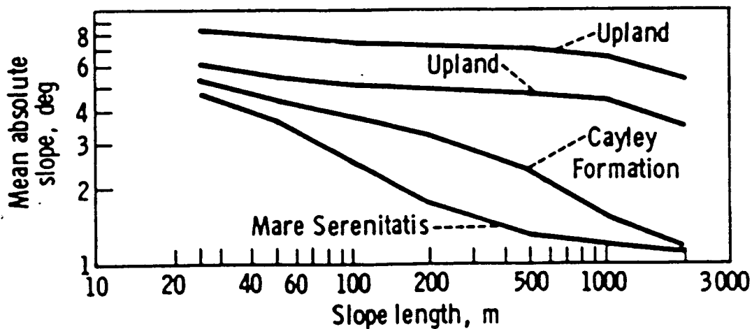
Figure 2.1-1, Lunar Slope-Frequency Distributions
