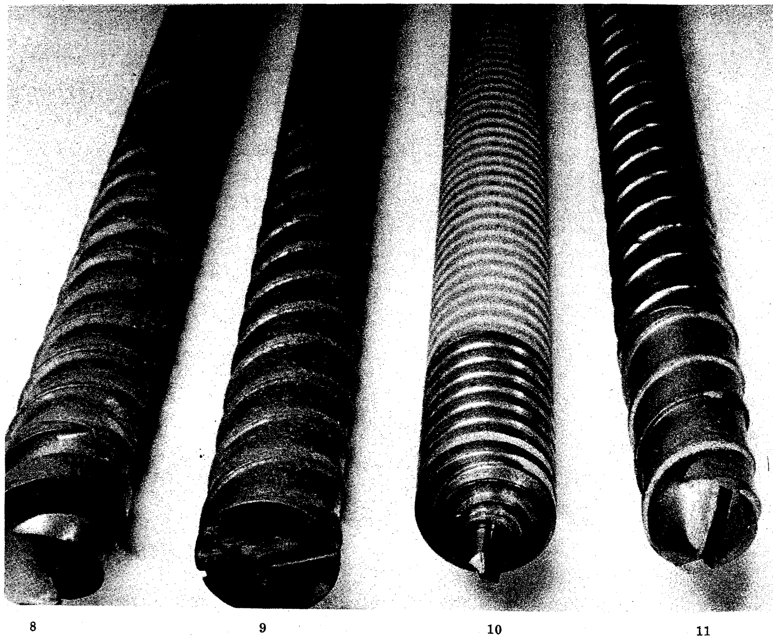
Figure III-9 Hole Casing Tip Configurations (Sheet 3 of 3)
