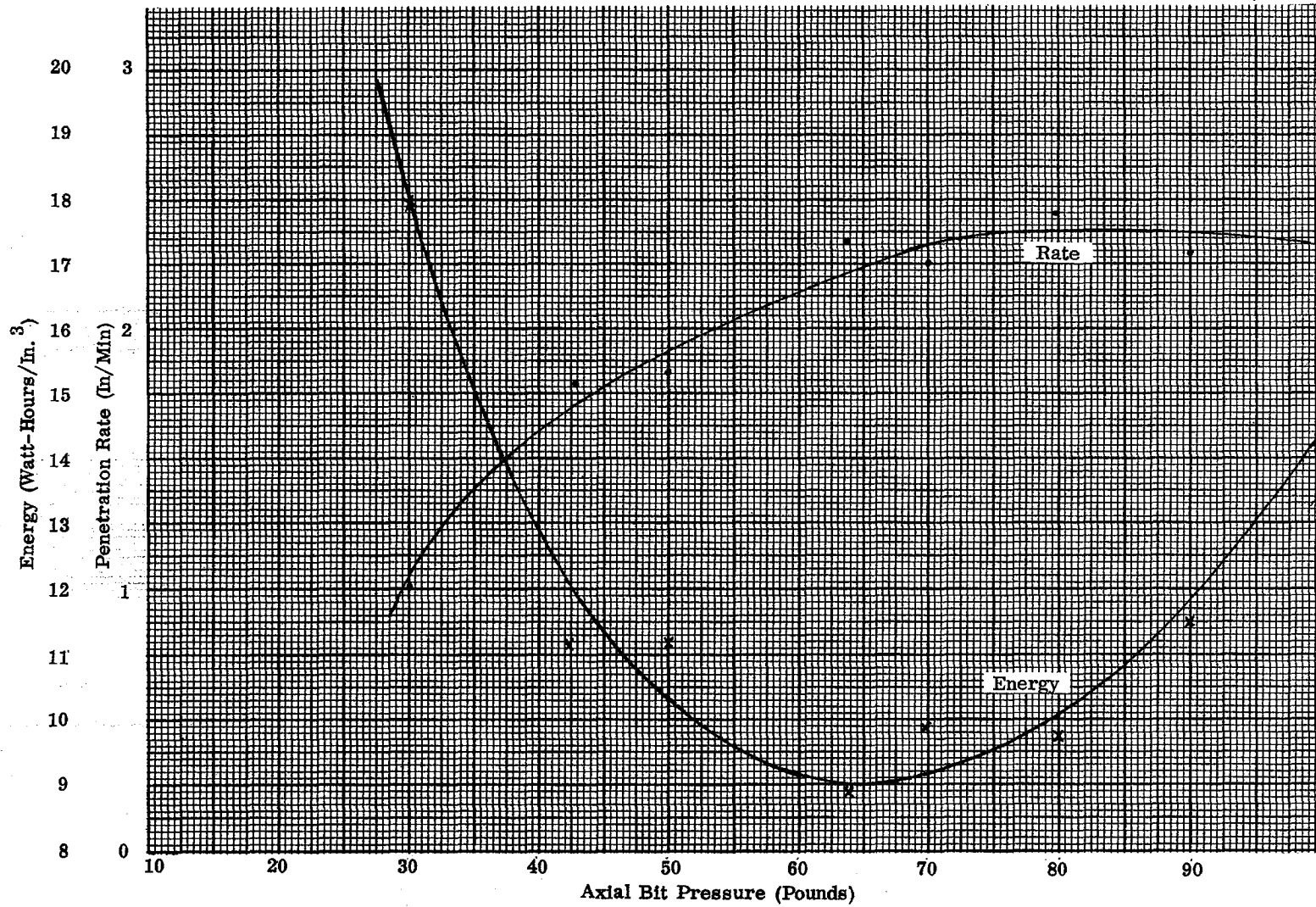
Figure III-4 ALS Performance Characteristics in NASA Standard High Density Basalt
