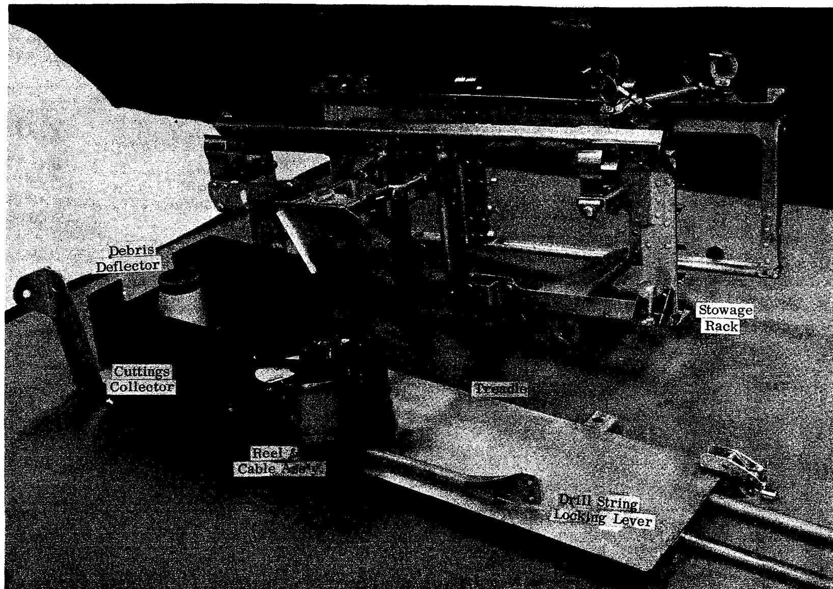
Figure II-9 Development Model Treadle Assembly.
