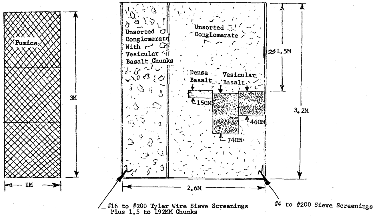
Figure III-24 3-Meter Conglomerate and Pumice Model Construction
