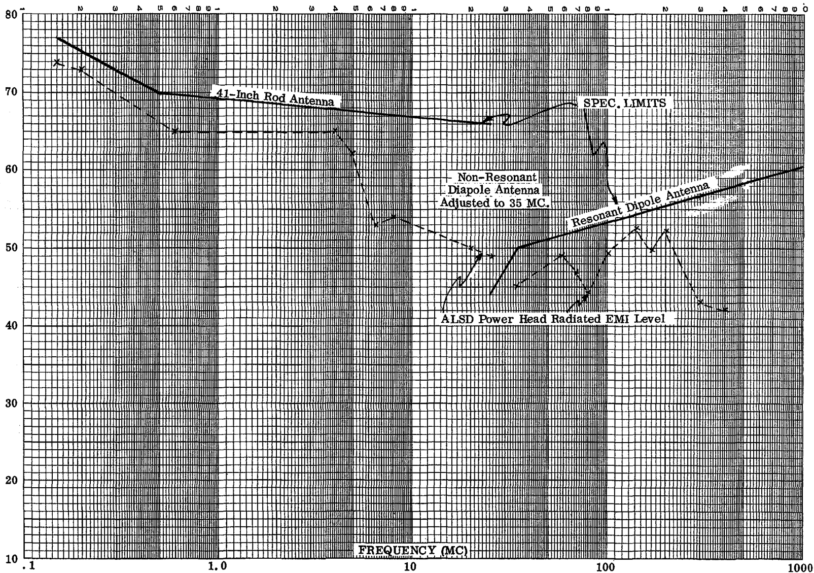
Figure III-12 Class I Radiated EMI of ALS Power Head (EMI Model)
