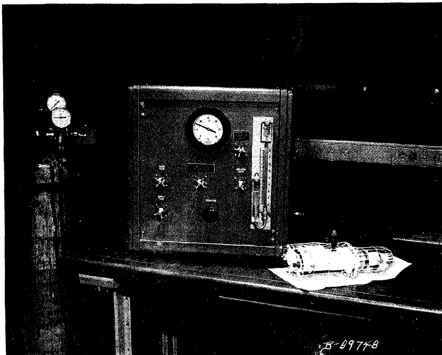
Figure 1-5 ALSD Pressurization Unit
