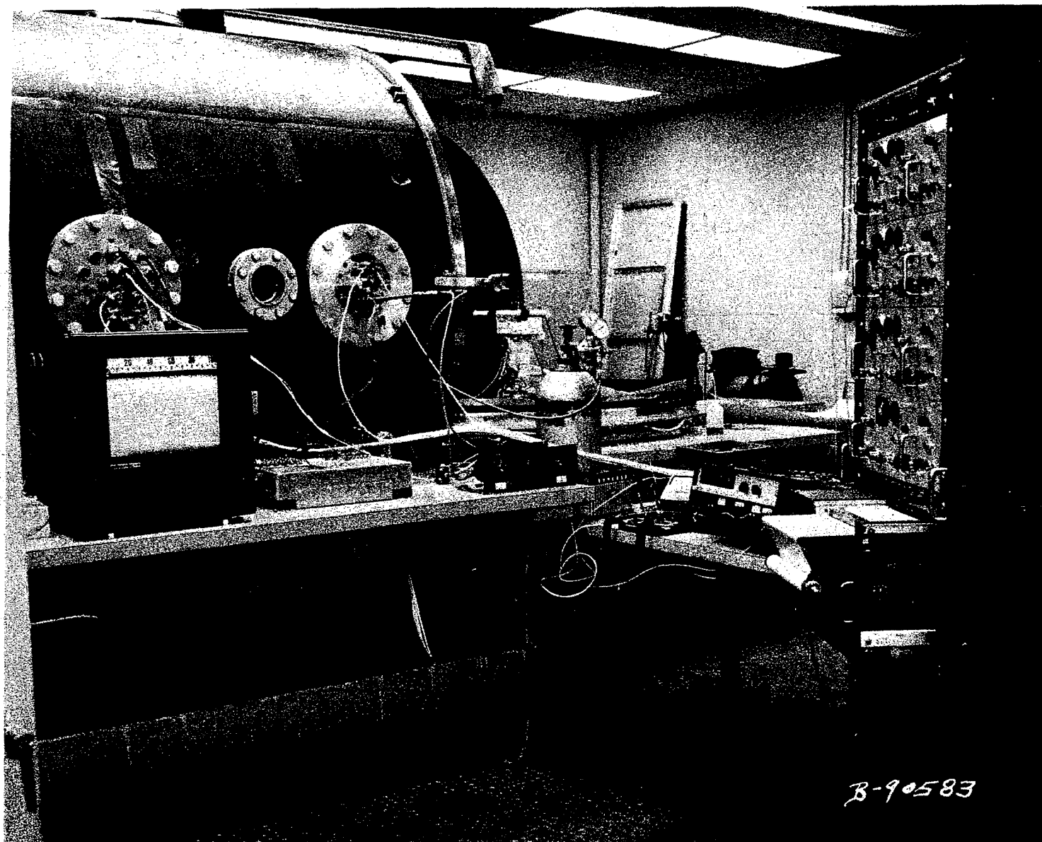
Figure IV-6 ALSD Thermal-Vacuum Test Equipment
