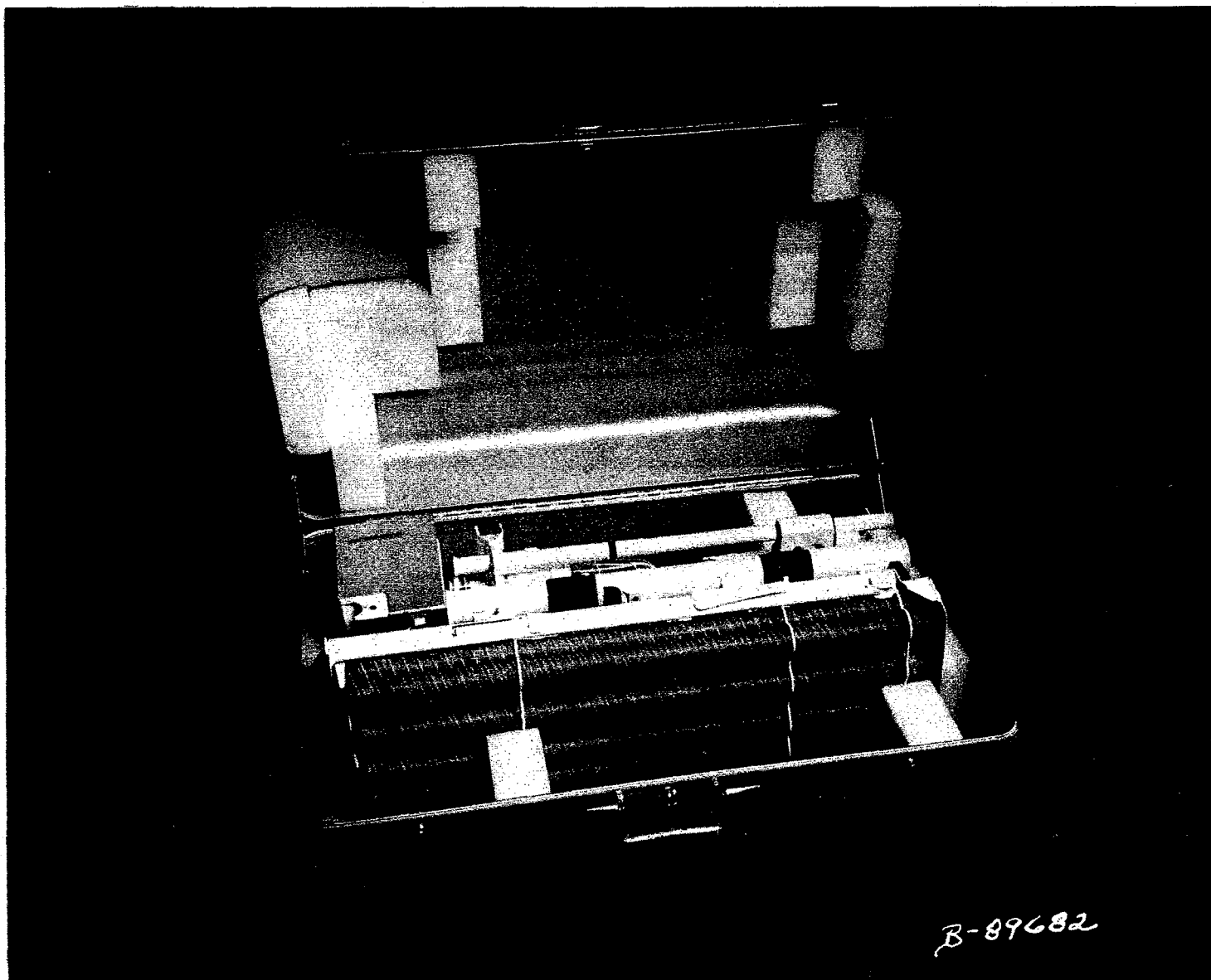
Figure I-2 ALSD Shipping Container
