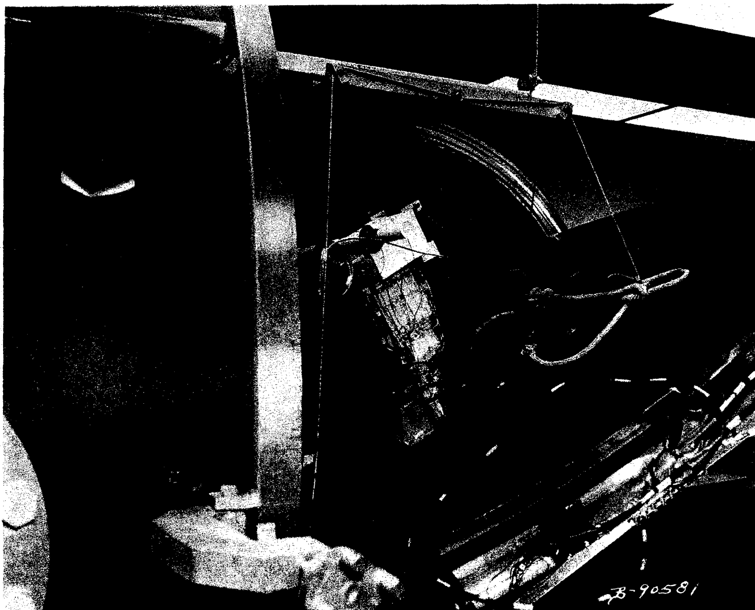
Figure IV-8 ALSD Operational Mode on Lunar Surface Simulator
