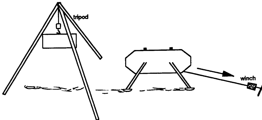
Figure 6-7b. Unloading Lander using Tripod
