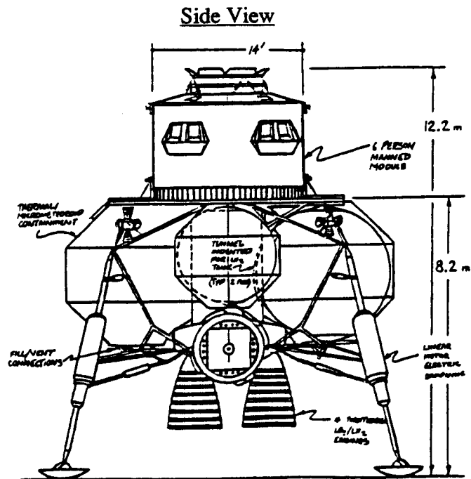
Figure 3-1. Single Stage \text{LO}_2/\text{LH}_2 Reusable Lunar Lander (Ref.3)
